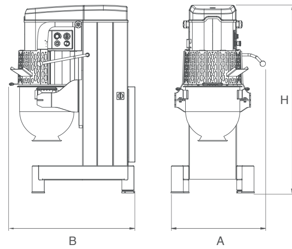
Dessins techniques C-Line 2 40/60/80
